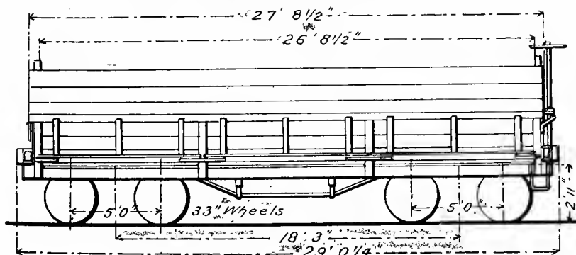
Fig. 71. Side Elevation.
